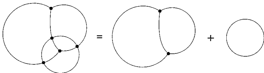
Figure 5: It is sometimes possible to place lower bounds on the length of a bubble by decomposing it into simpler pieces. The bubble on the left may be decomposed into a standard double bubble and a single bubble.
