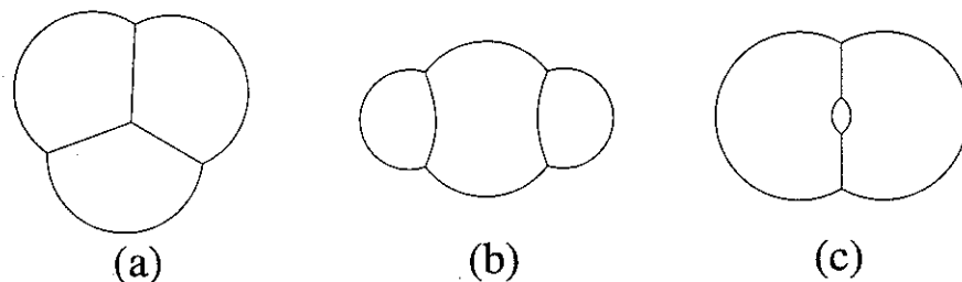
Figure 3: We first show that any length-minimizing enclosure of three connected areas has one of these three combinatorial types.
