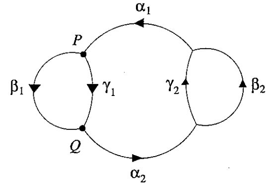
Figure 11: Lemma 8.1 shows that \alpha_1 and \alpha_2 lie on the same circle or line. These edge labelings are used in the proof of Proposition 8.2, where we show that in nondegenerate, length-minimizing, overlapping bubbles of type (b), edges do not overlap.
