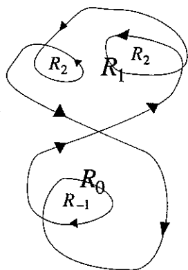
Figure 10: \gamma can be decomposed into boundaries of regions R_i .
