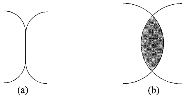
Figure 4: When we allow regions to overlap, bumped-up curves revert to constant-curvature arcs.
