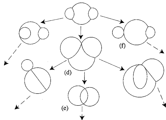
Figure 14: The first few degeneracies of type (b).
