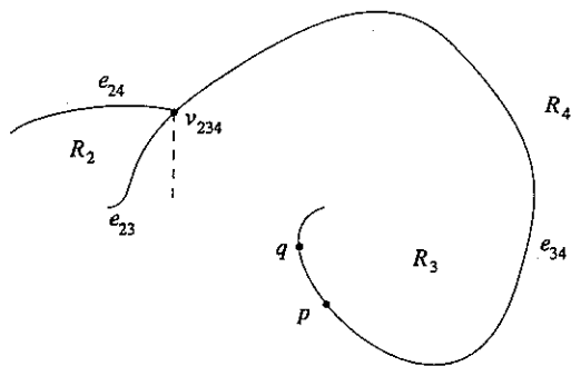
Figure 9: e_{23} and e_{34} cannot bump.
