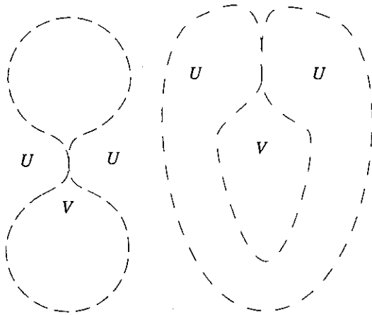
Figure 7: The two possibilities when two points of \gamma merge with V between them.
