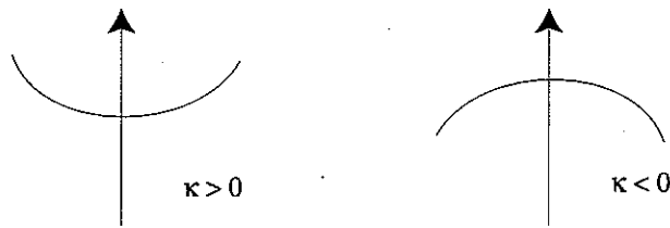
Figure 6: Sign conventions for the oriented curvature of an edge crossed by a path.
