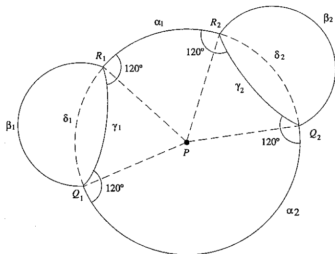
Figure 13: Edges \gamma_1 and \gamma_2 of bubble B cannot intersect because they are separated by the two dotted triangles.
