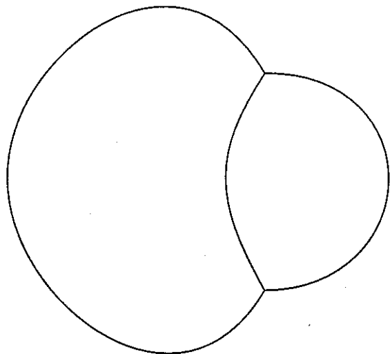
Figure 1: The standard double bubble in \mathbb{R}^2 is uniquely length-minimizing.
