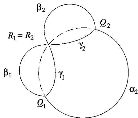
Figure 15: Bubble B' has the same length and encloses the same areas as bubble B of Figure 13, but is not of allowable type; hence B is not length-minimizing.
