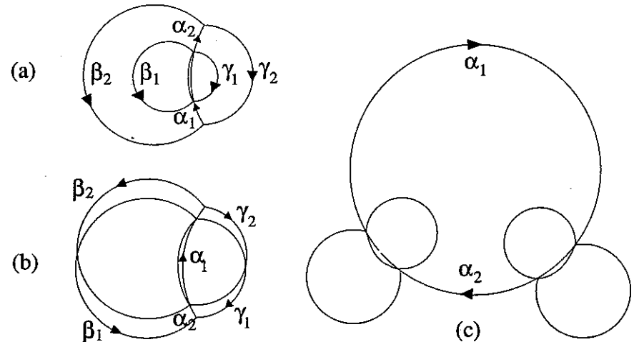
Figure 12: Different ways in which \alpha_1 and \alpha_2 might overlap.
