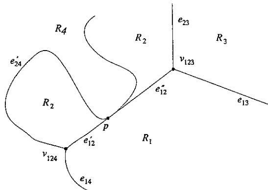
Figure 8: If e_{12} and e_{24} bump, then e'_{12} cannot bump e_{23} .
