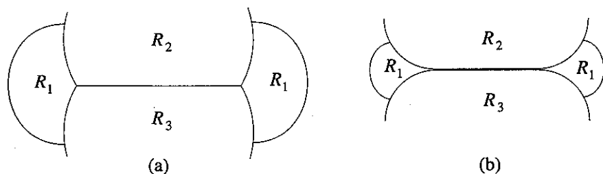
Figure 2: (a) In general, regions may be disconnected. (b) In the connected regions problem the regions may be connected only by "infinitesimal strips".
